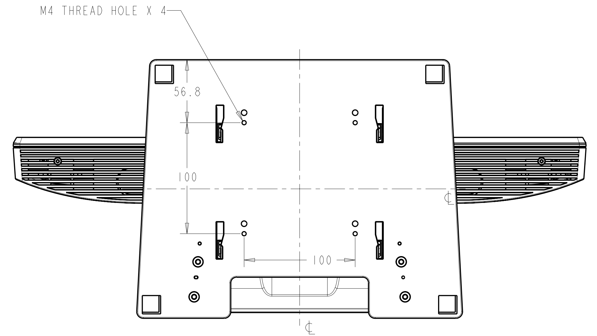
BOTTOM VIEW
