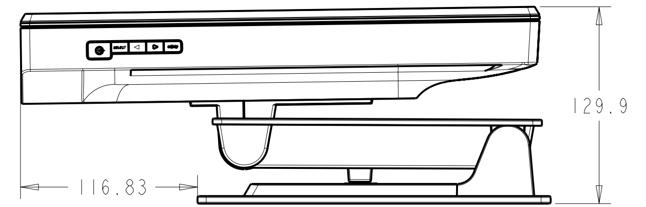
MONITOR FULLY COLLAPSED
