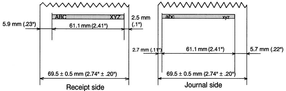
Figure 1.9.1 Paper Roll Printable Area
