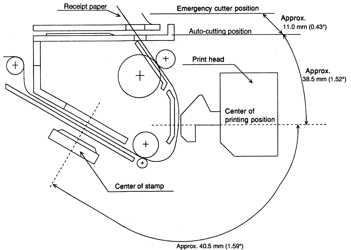
Figure 1.10.1 Printing, Stamp, and Auto Cutter Positions
