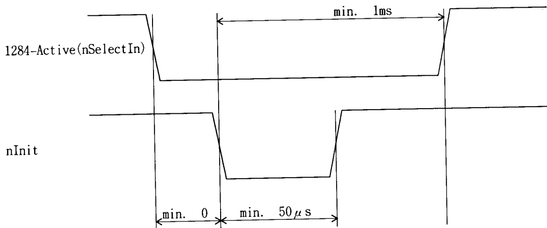
Figure J.2.2.1 nInit signal-driven hardware reset
