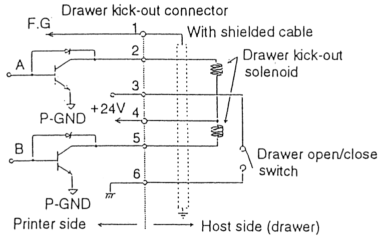
Figure 2.2.3 Drawer Circuitry
