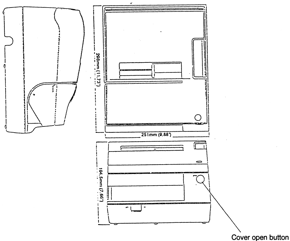
Figure 4.3.1 External Appearance
