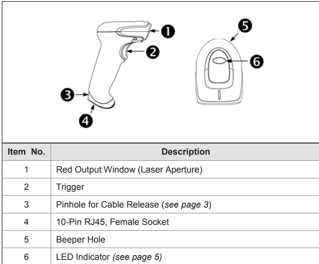
Figure 1. Scanner Components
